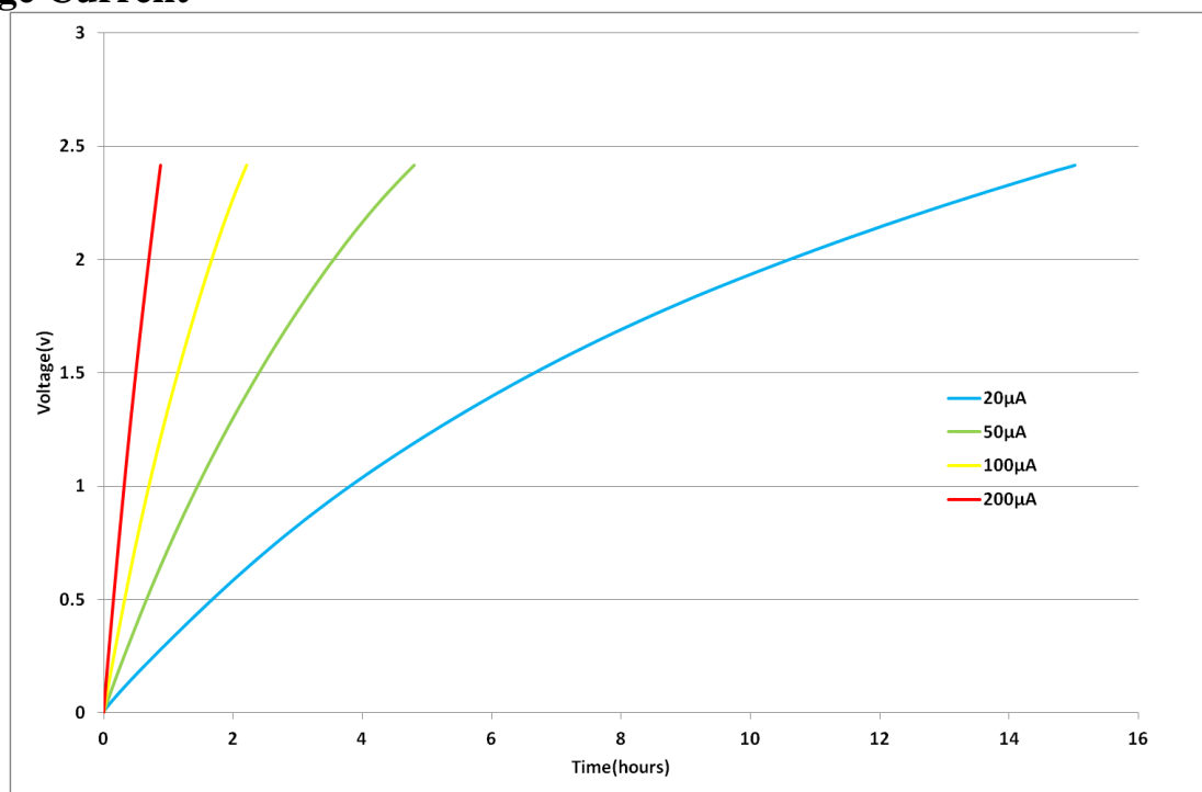
Fig 11: Charging an HA102 with low current
